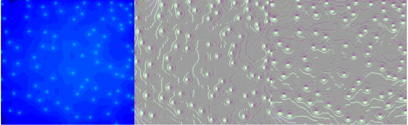
Illustration 10: Experimental direct integration RBF applied to electrostatics, this pattern resulting shortly after release of a random initial distribution into a vacuum. From left to right: Electrostatic potentials around each RBF node center, force field in the x-direction, force field in the y-direction. At equilibrium potential gradients at each node are zero, and where not, gradients from neighboring contributions resulting in local acceleration. Iso-potential contours are naturally apparent between nodes, with radius of influence a function of stencil size and resulting spatial accuracy / smoothness..
