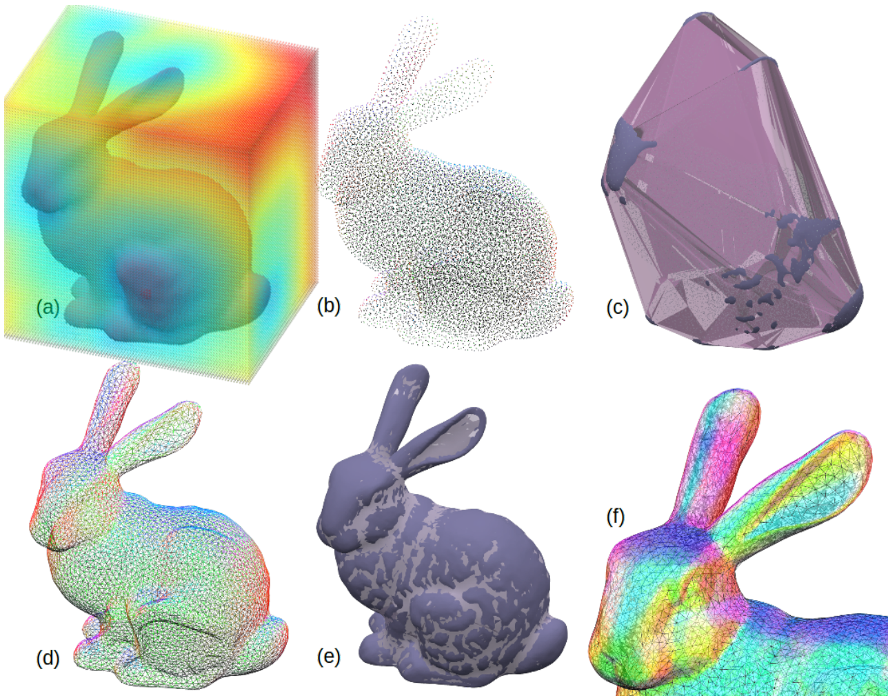
Illustration 9: Stochastic meshing process with 20K nodes, unrefined: a) Shape is defined by reference surfaces used to solve SDF background. b) Nodes are injected into valid SDF locations and equalized. c) Triangulation updates topology with over-wrapped mesh (comprised of convex hulls). d) Elements are evaluated and cleaned against SDF while surfaces are unwrapped. e) Original (darker) mesh superimposed over new mesh to visualize spatial deviation. f) Close-up showing error around high-curvature features.
