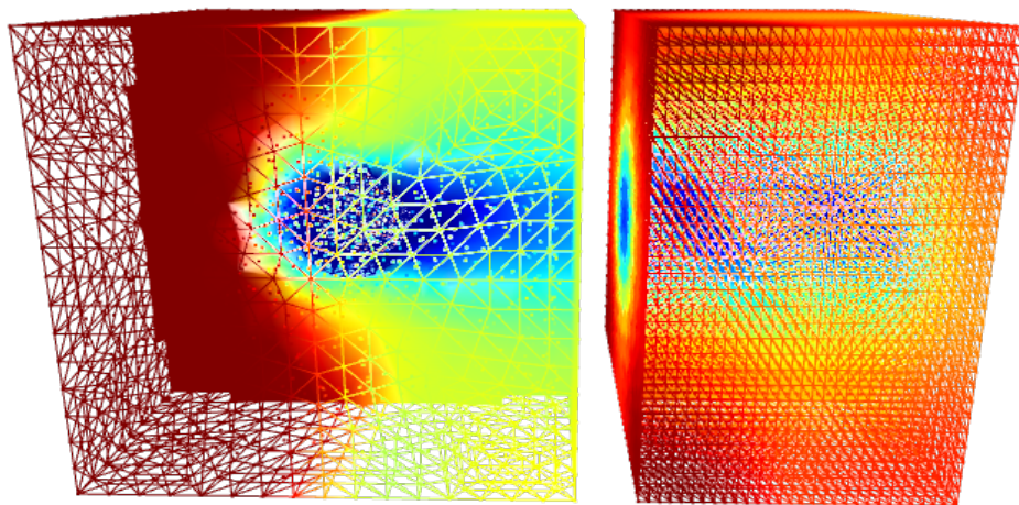
Illustration 5: Inter-domain mutual coupling between disparate geometry types. Unstructured mesh on left, structured grid on right, running two independent numerical methods coupled in time and space. In this test, a cylinder is placed inside a gas flow, with wake clearly visible through domains. Inter-operable algorithms enable higher-level coupling and global accuracy.
