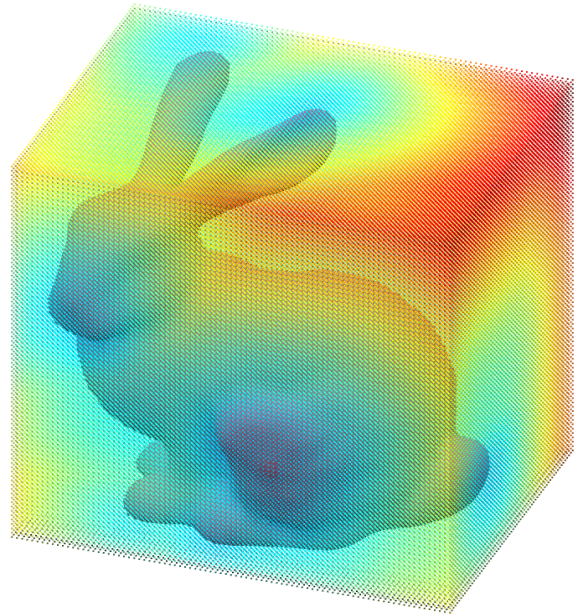
Illustration 11 SDF background field around reference surfaces defined by discrete triangles or analytic functions. An explicit representation can be converted into a discrete implicit field by first solving a narrow shell, followed by fast marching or viscosity solver to approximate the eikonal field. Fully-procedural constructive solid geometries are possible by defining the SDF field as primitives and operators to be evaluated a late stage, such implicit ray-tracer. RBF and other compression transforms possible.
