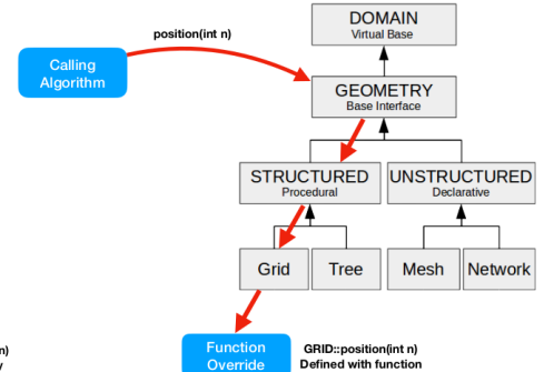
Illustration 3: Example grid position function override specialization, redirecting generic call to return values dynamically generated by local function. This may increase processing overhead, but minimize IO traffic.
