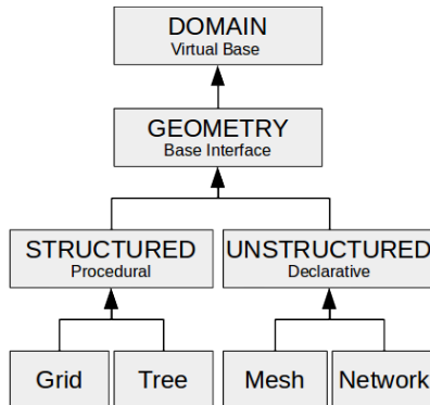
Illustration 1: Geometry Type Taxonomy. It is posited such inheritance and resulting polymorphism can support a standard common programming interface and optimizations for any type.
