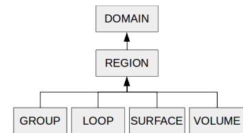
Illustration 14: Region Inheritance
