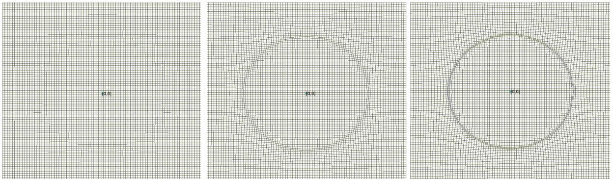
Illustration 7: Tensor morphing to resolve circle in structured grid. Left to right: 1x, 2x, 4x refinement. Different morphing algorithms can yield varying degrees of skewness and orthogonality. To permit FDM and convolution on curvilinear grids, operators must transform and de-transform by Jacobian \partial x_i/\partial \xi_j , a generalization not yet performed in our latest code.
