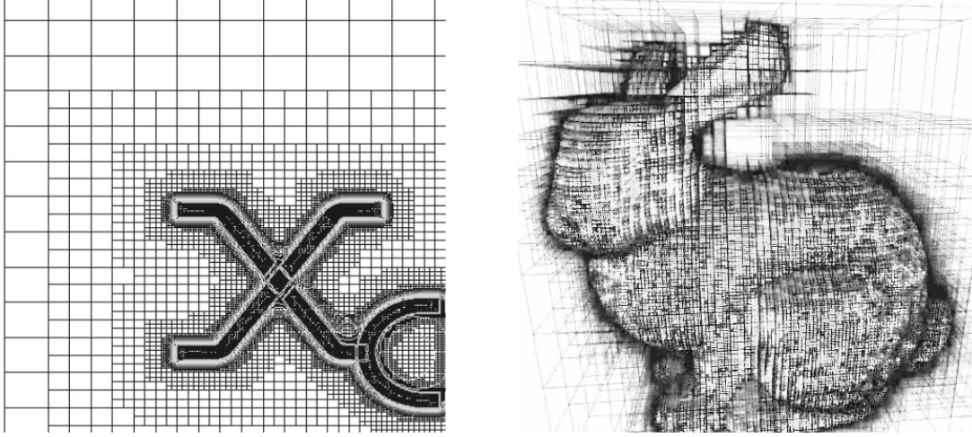
Illustration 8: Examples of trees in 2d and 3d. Left, prototype quadtree demonstrate growth layers around discrete shape. Right, octree (container) improves search space during mesh winding-number calculation. High-performance procedural tree geometries are possible and will be a workhorse in emerging CAE analyses.
