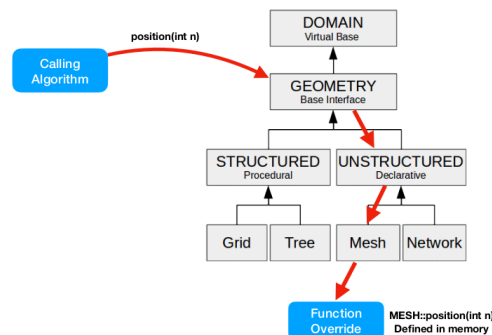
Illustration 2: Example mesh position function override specialization, redirecting generic call to return values statically stored in memory. This may minimize processing overhead, but also increases IO traffic.
