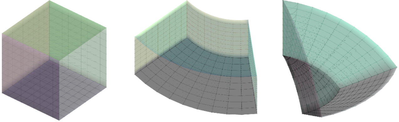
Illustration 6: Simple orthogonal grids of size IJK[10,10,10], from left to right: Cartesian, cylindrical, spherical isometries with min[1,0,0] & max[2,1,1]. This particular example demonstrates a regional degeneracy on the spherical surface k+ .
