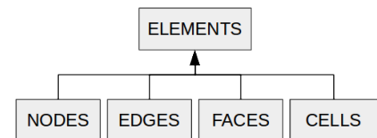
Illustration 13: Elements Inheritance
