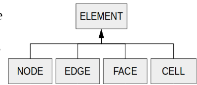
Illustration 12: Element Inheritance
